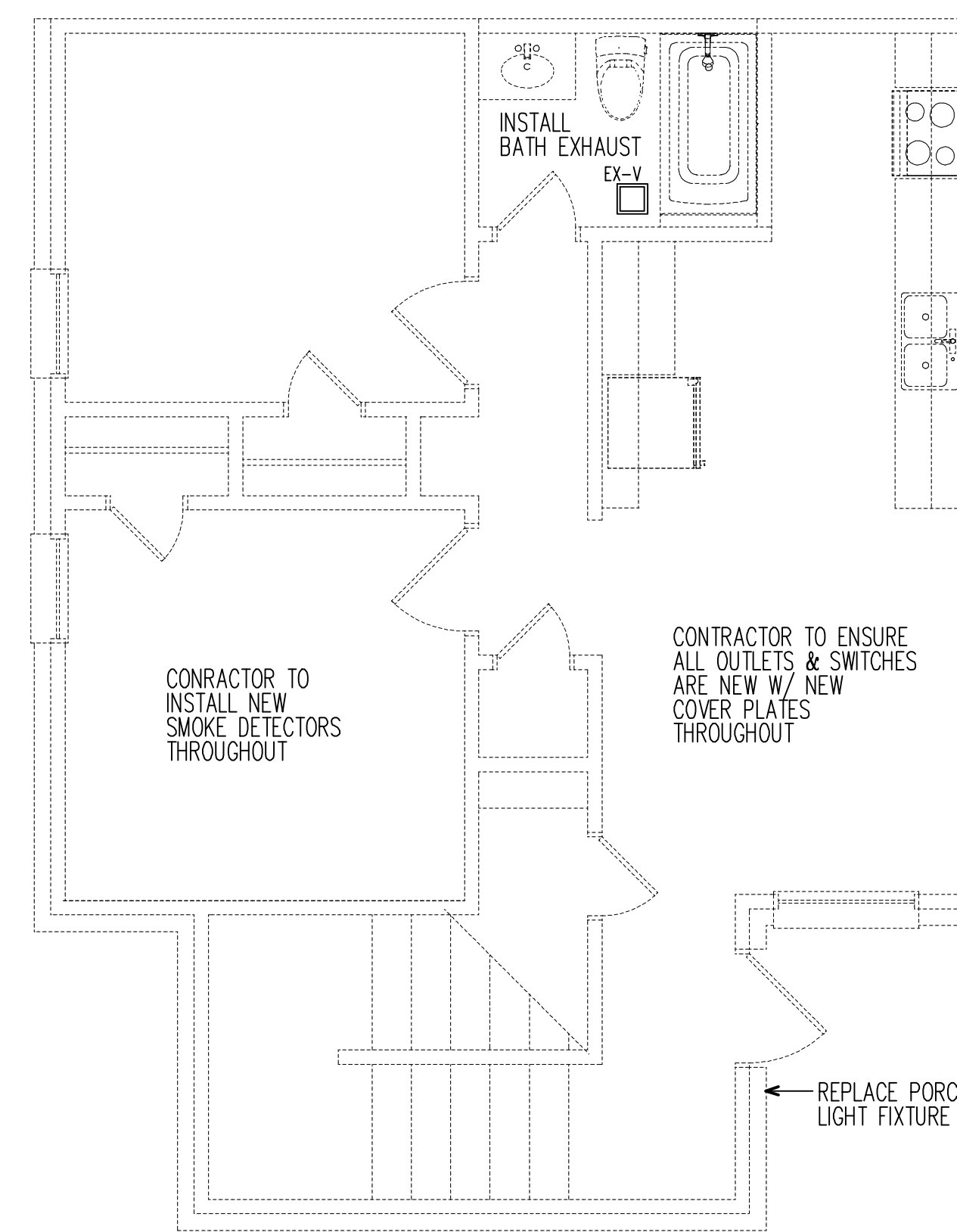
03 UNIT 208 - 1ST.FL. RCP SCALE: 1/4" = 1'-0" 4-BEDROOM TYPE
