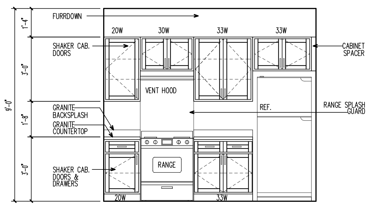
04 KITCHEN ELEV. @ RANGE/REF. SCALE: 3/8" = 1'-0"
