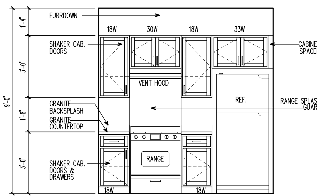
04 KITCHEN ELEV. @ RANGE/REF. SCALE: 3/8" = 1'-0"
