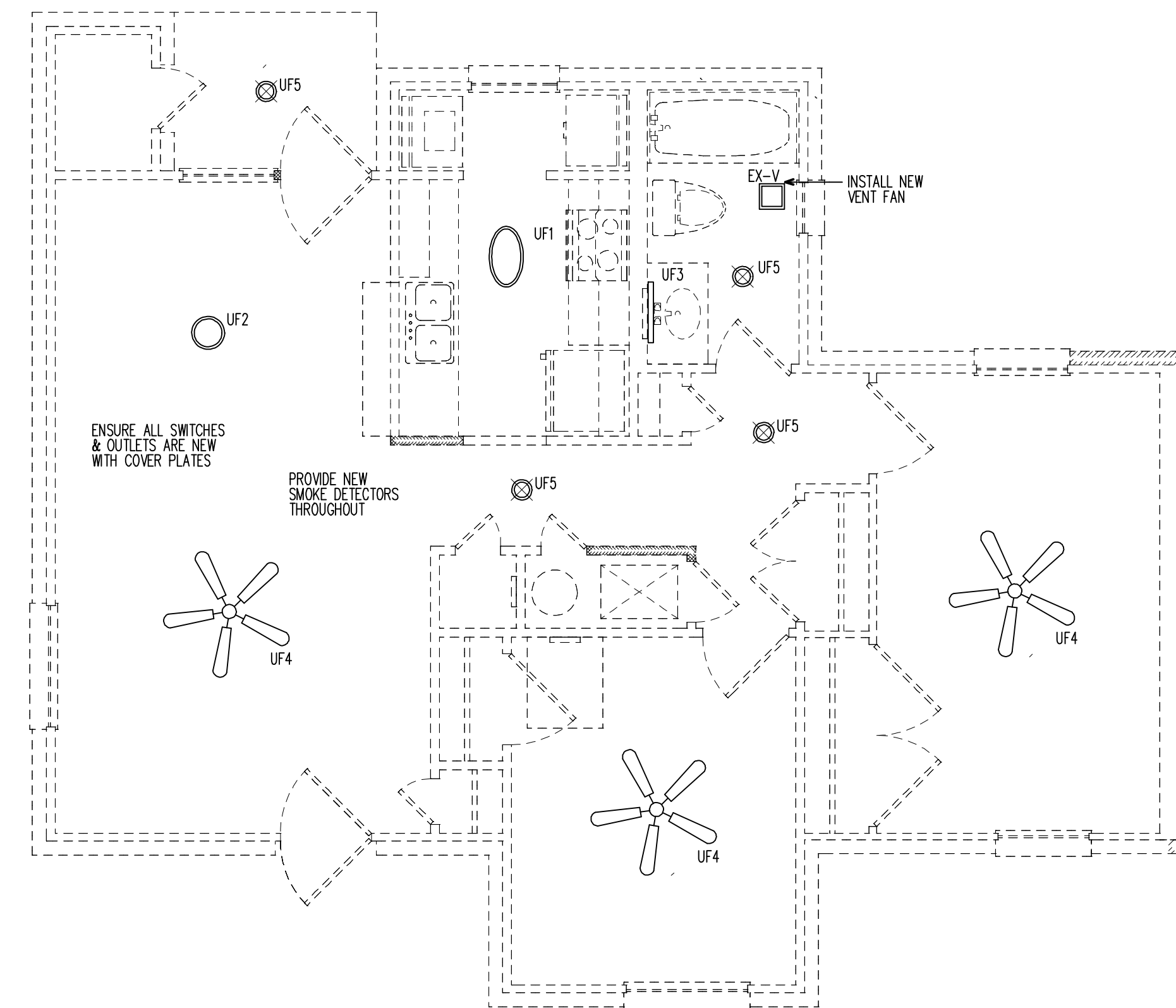
01 REFLECTED CEILING PLAN SCALE: 1/4" = 1'-0" UNIT D6
