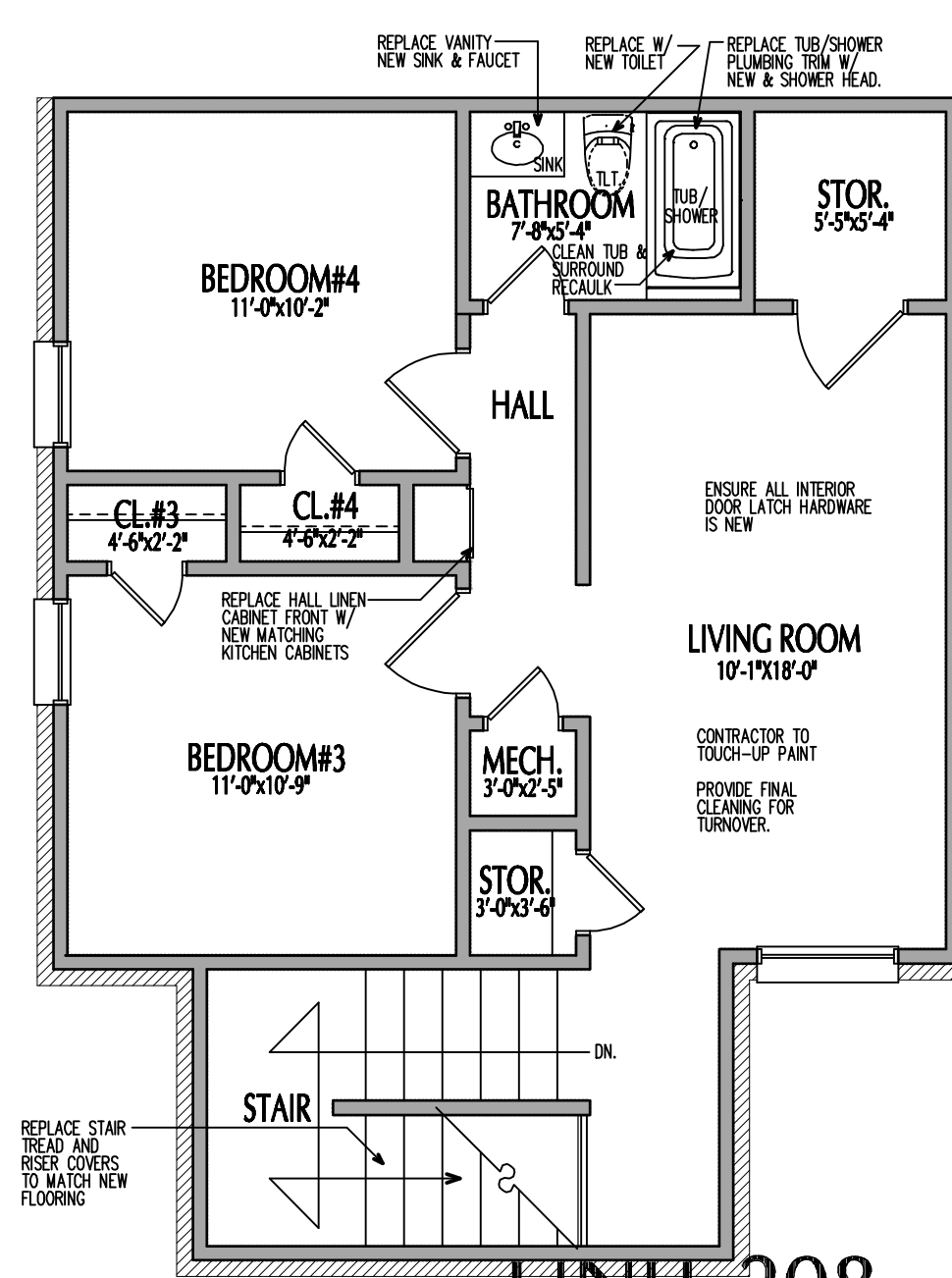
02 UNIT 208 - SECOND FLOOR PLAN SCALE: 1/4" = 1'-0" 4-BEDROOM TYPE
