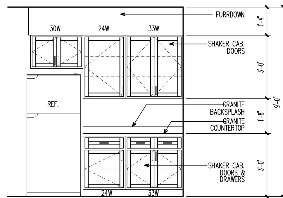
07 KITCHEN @ REFR. SCALE: 3/8" = 1'-0"
