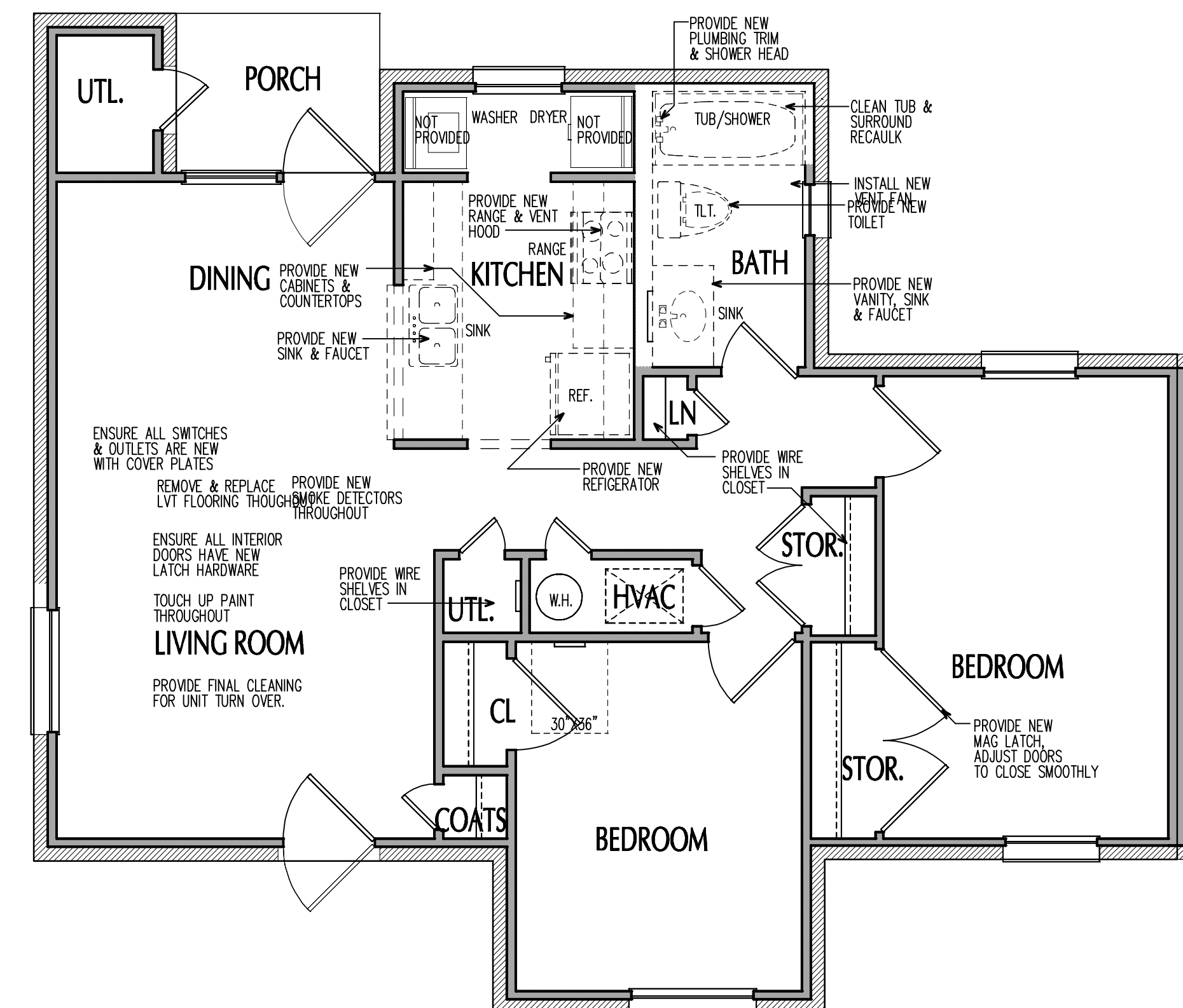
02 FLOOR PLAN "F2" - RENOVATION SCALE: 1/4" = 1'-0" UNIT D6
