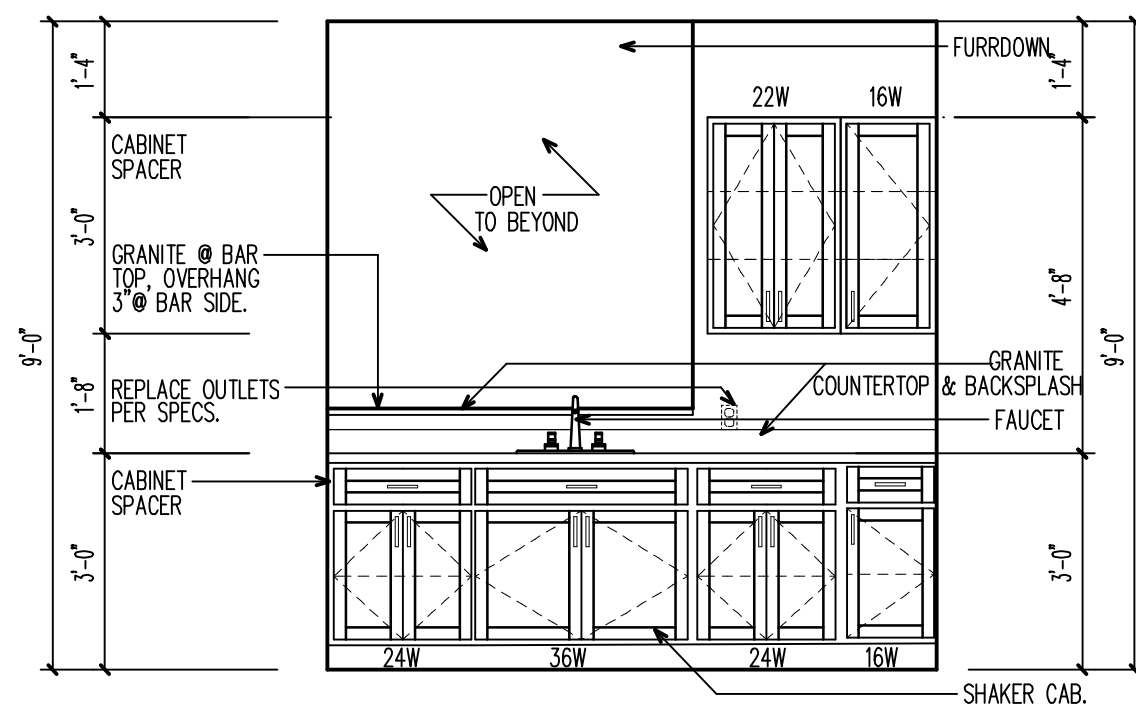
03 KITCHEN ELEV. @ SINK SCALE: 3/8" = 1'-0"
