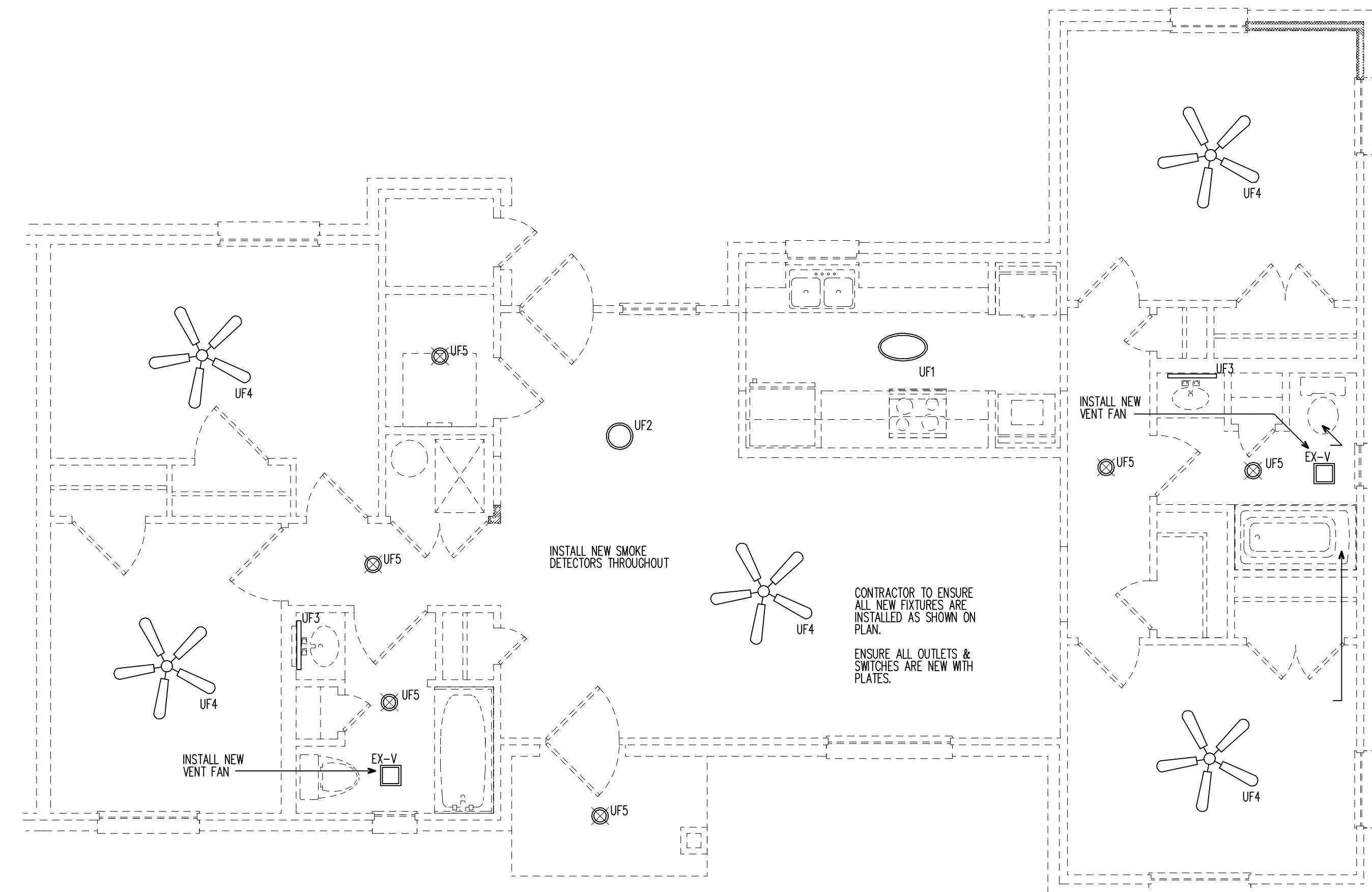
01 REFLECTED CEILING PLAN SCALE: 1/4" = 1'-0"
