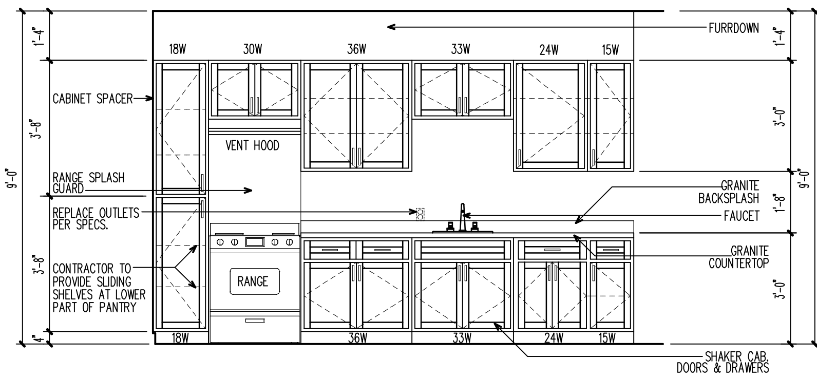
06 KITCHEN @ SINK/RANGE SCALE: 3/8" = 1'-0"
